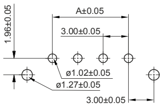
RECOMMENDED HOLE PATTERN
