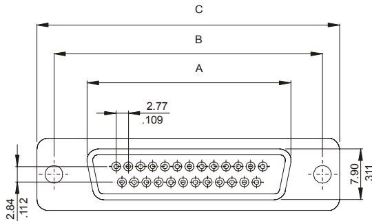
9 to 37 Circuits
