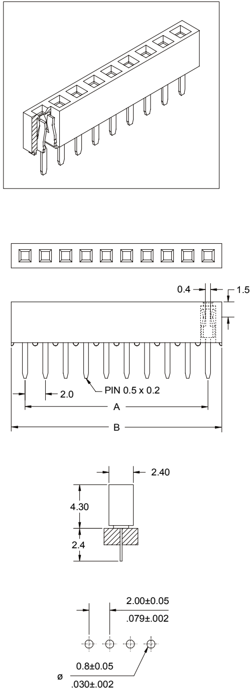
RECOMMENDED HOLE PATTERN
