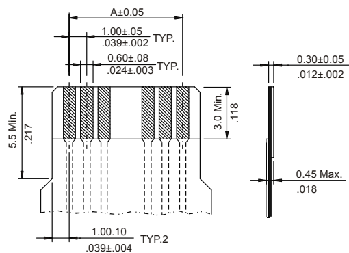
* ACCOMMODATED FPC
