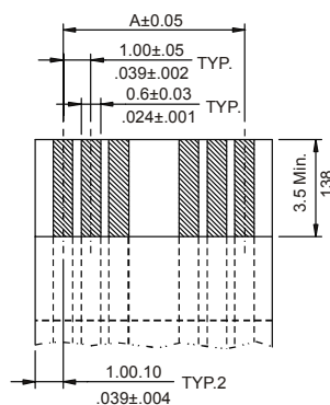
* ACCOMMODATED FFC
