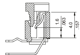
Upside contact
