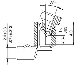
Downside contact
