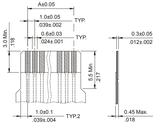
ACCOMMODATED FPC
