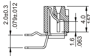
Downside contact
