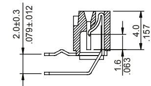
Upside contact
