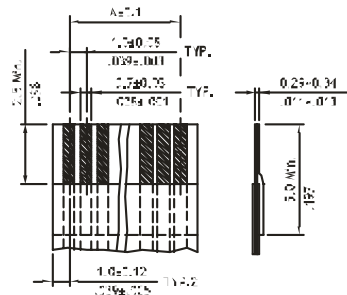
Accommodated FFC/TPC
