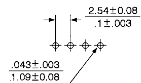
RECOMMENDED HOLE PATTERN
