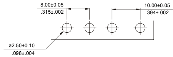
RECOMMENDED HOLE PATTERN
