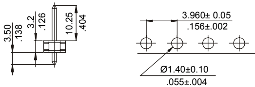
RECOMMENDED HOLE PATTERN
