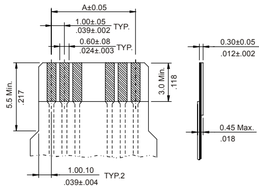
* ACCOMMODATED FPC
