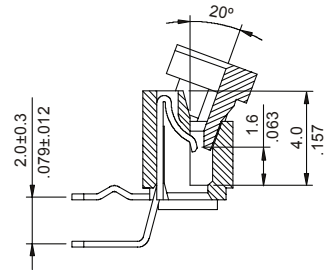
Downside contact
