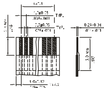
Accommodated FFC/TPC
